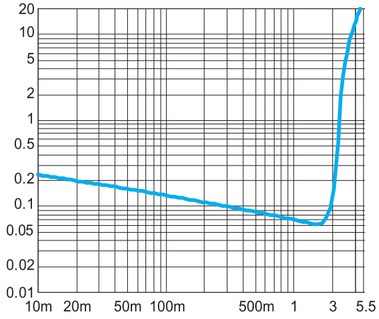
THD+N vs. Output Power 4.2V, 40ohm, f=1 kHz
