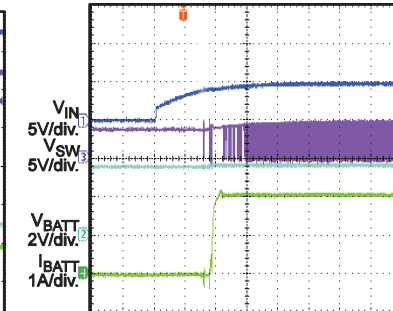
Power On V_{BATT} = 3.6V
