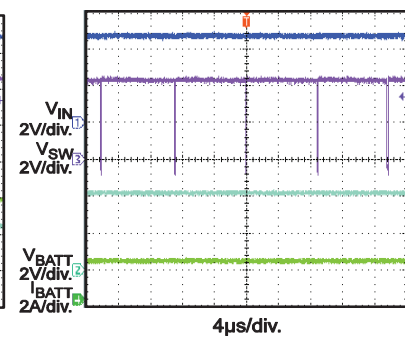
Power OFF V_{BATT} = 3.6V
