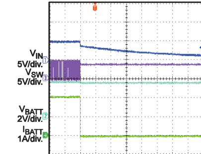
Power OFF V_{BATT} = 3.6V
