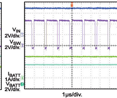
Power On V_{BATT} = 3.6V
